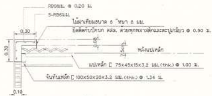
DETAIL ① SCALE 1 : 20
