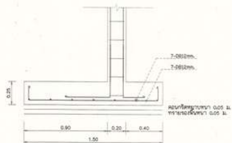
Fo Scale 1:20
