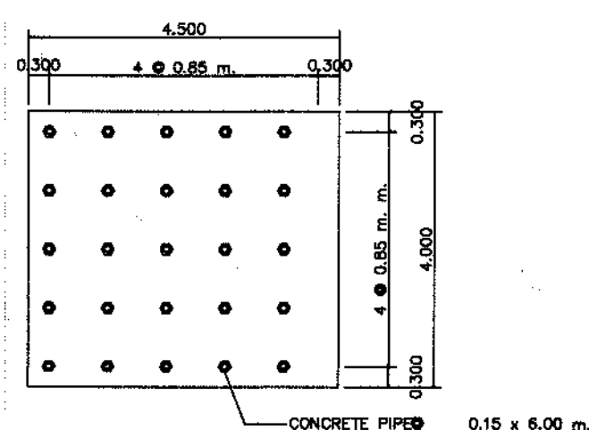
PLAN OF FOUNDATION SCALE: 1:100
