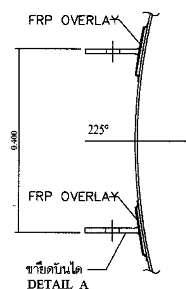
DETAIL A
