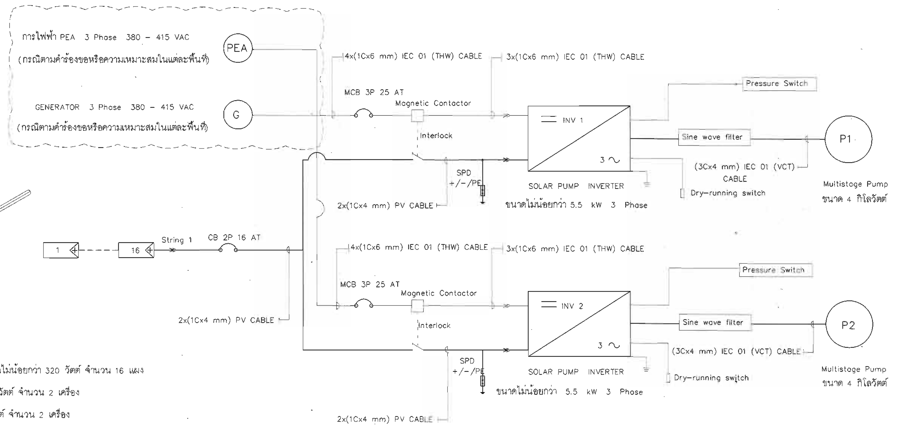
SINGLE LINE DIAGRAM
