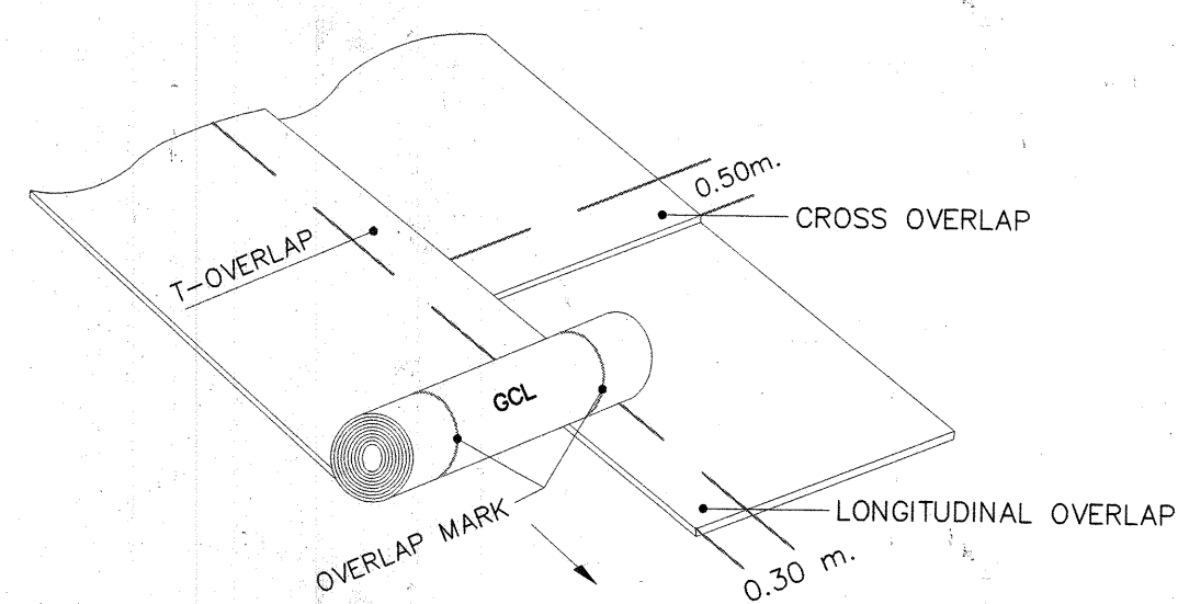
TYPICAL OVERLAP DETAIL NOT TO SCALE
