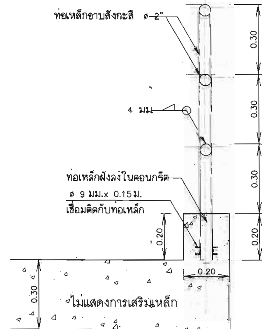
SECTION F - F 1:10
