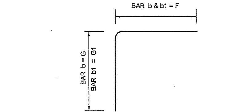
BENDING DETAILS FOR BARS b & b1 NOT TO SCALE
