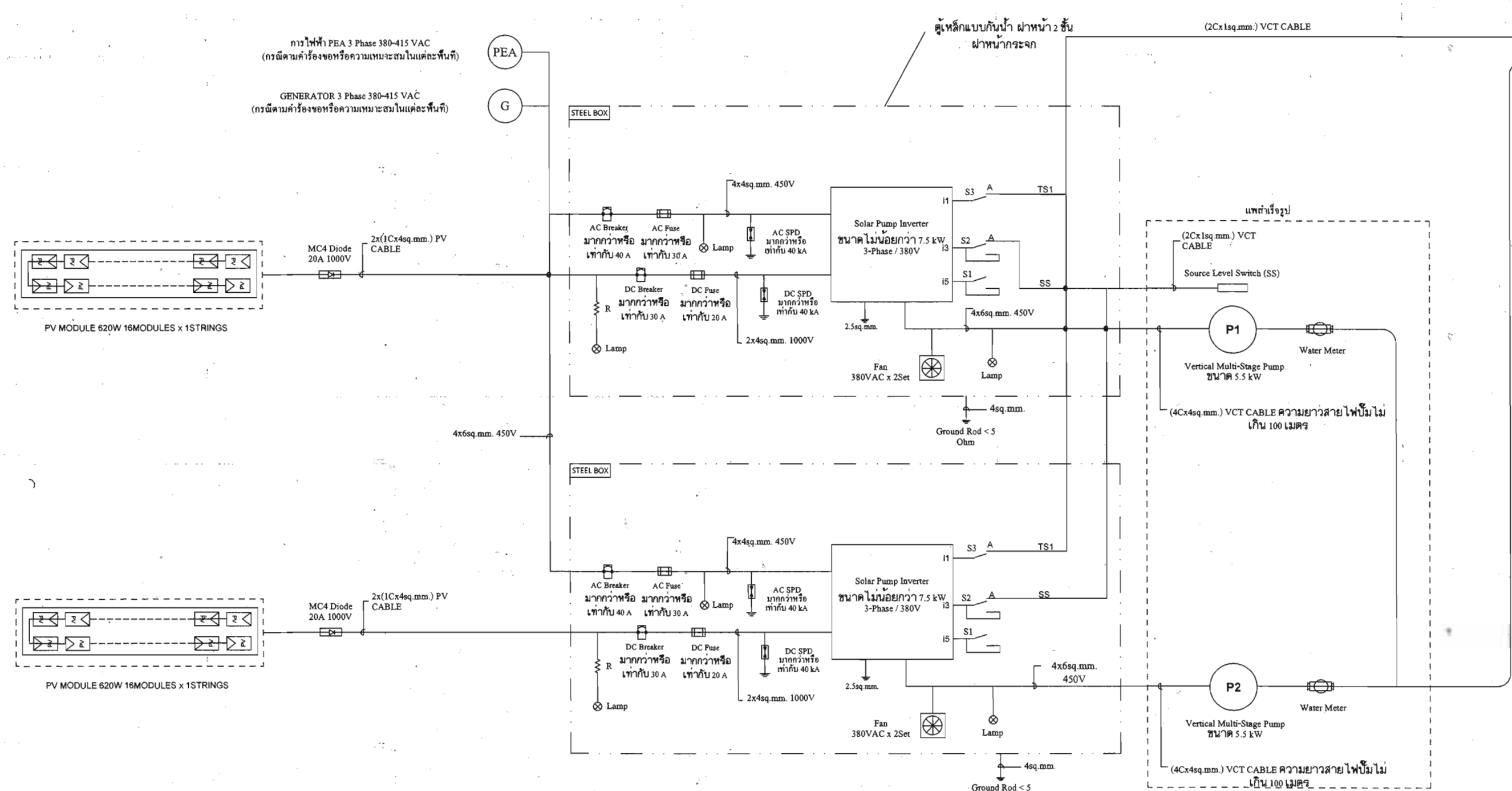
SINGLE LINE DIAGRAM (5.5kW-Pump x 2Units)
