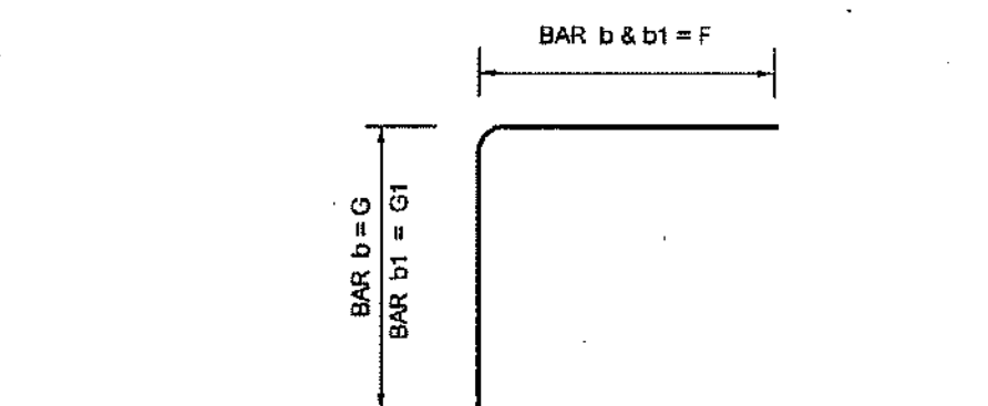
BENDING DETAILS FOR BARS b & b1 NOT TO SCALE
