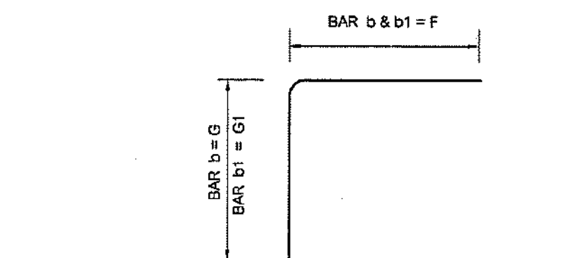
BENDING DETAILS FOR BARS b & b1 NOT TO SCALE
