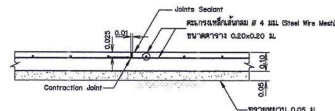
(Contraction Joint)
