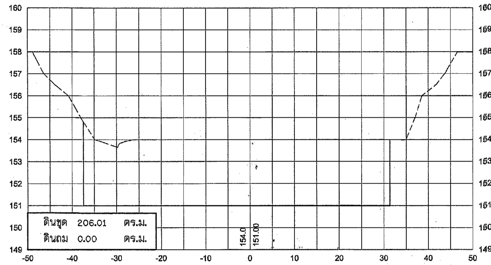
5+200
