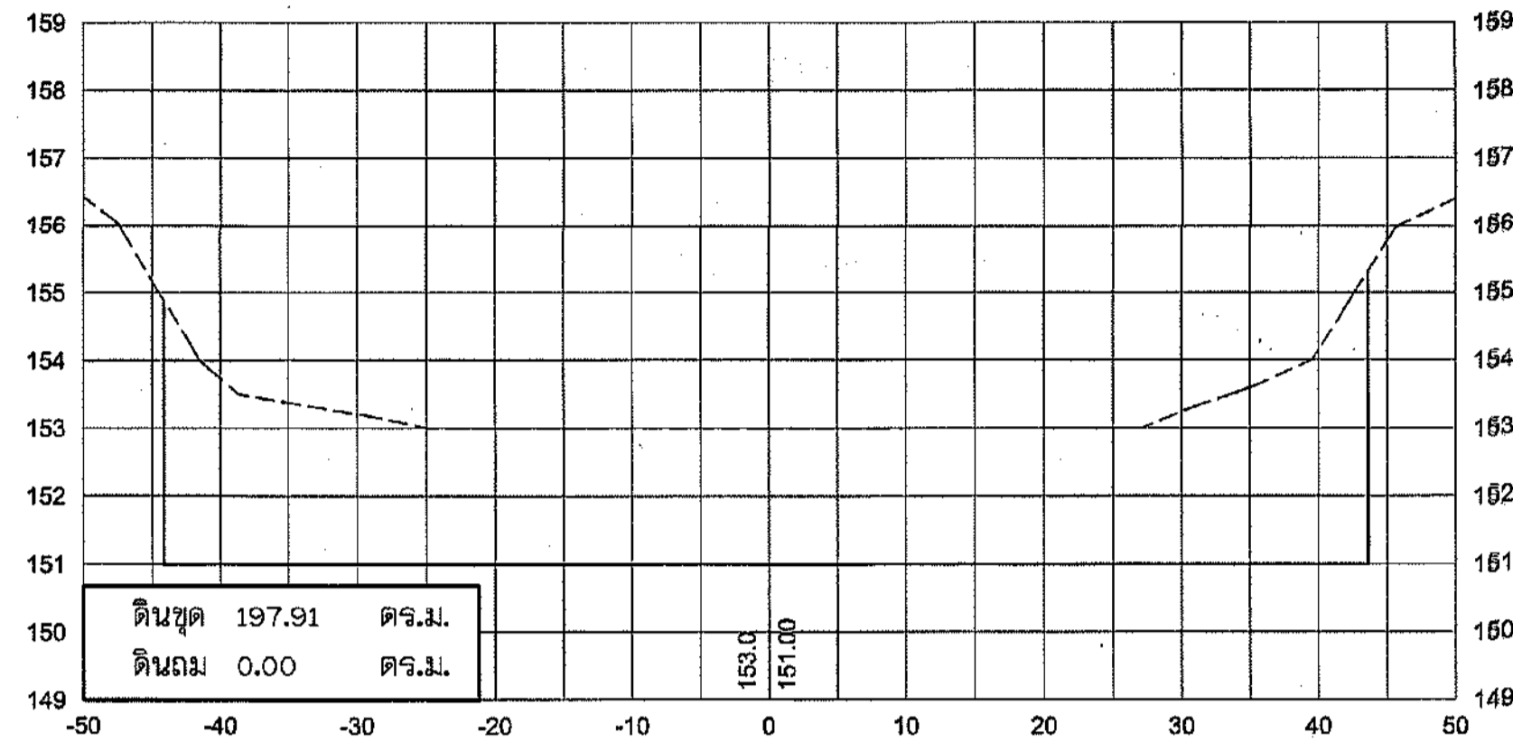
5+250
