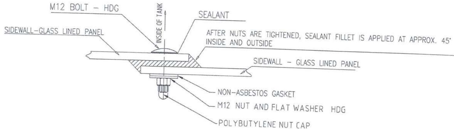
SIDEWALL SEALANT DETAILED
