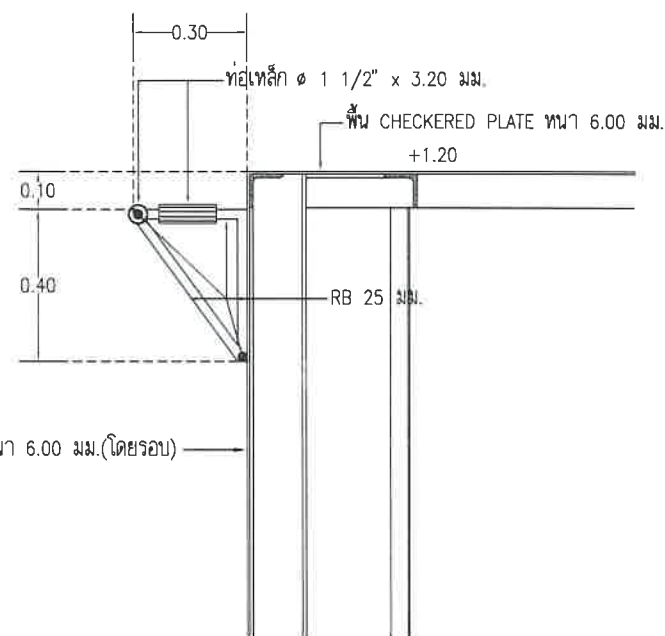
SECTION 1-1 SCALE 1:20
