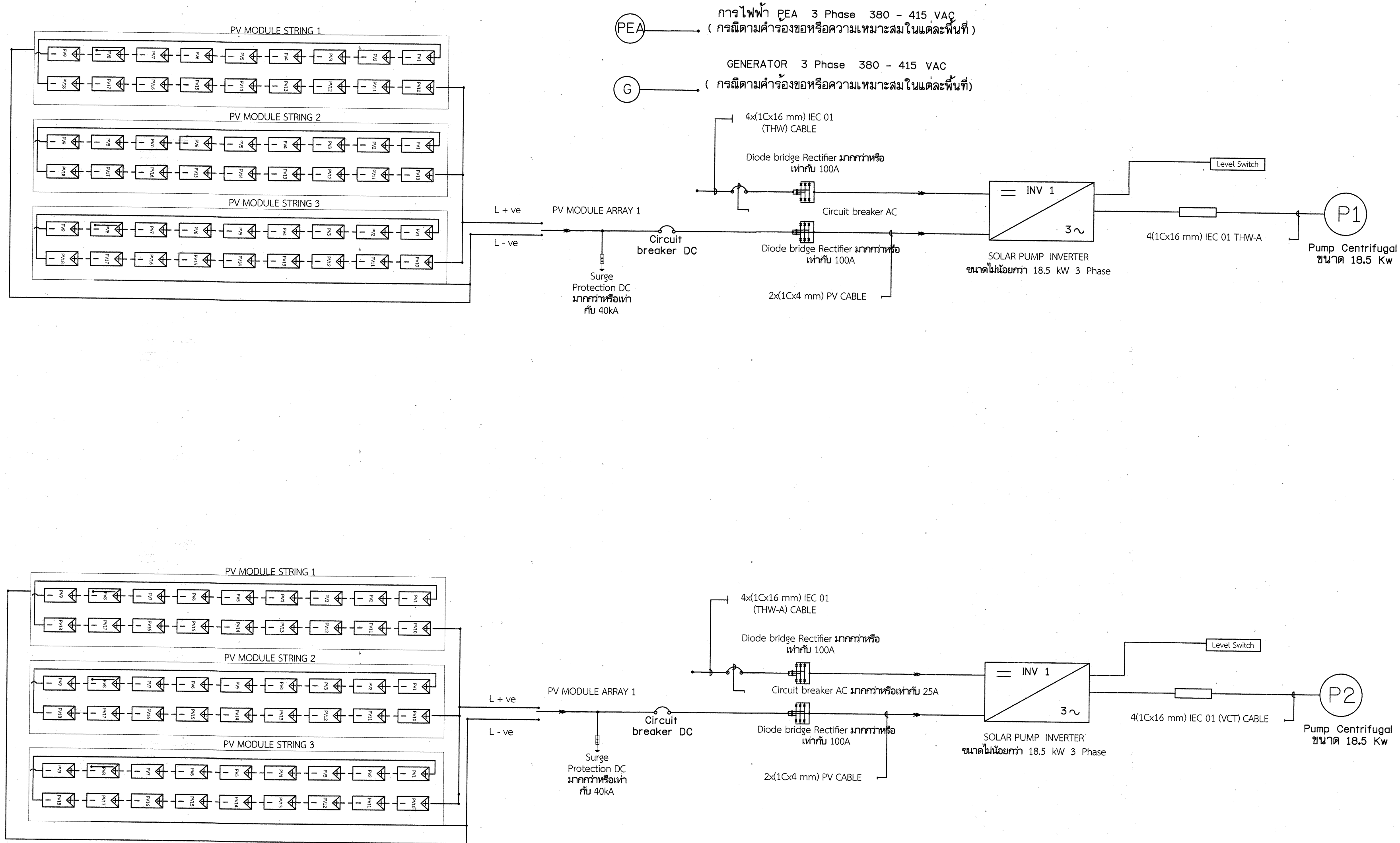
SINGLE LINE DIAGRAM
