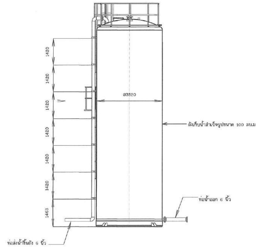
WATER STORAGE TANK MODEL SCALE 1:125
