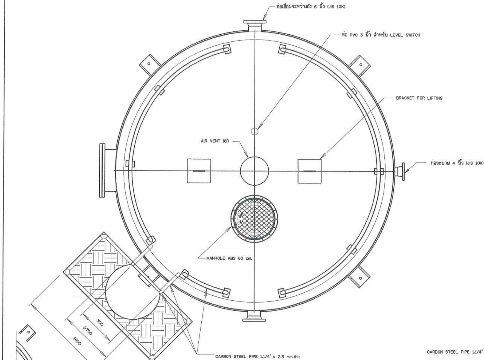
DETAIL TANK + LADDER SCALE 1:30
