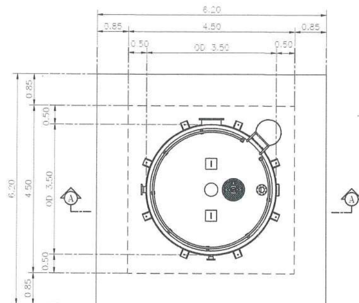
FOOTING PLAN (WTF-100000V-D3.50) SCALE 1 : 100
