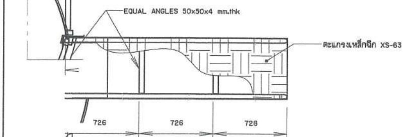
DETAIL TANK + LADDER SCALE 1:30
