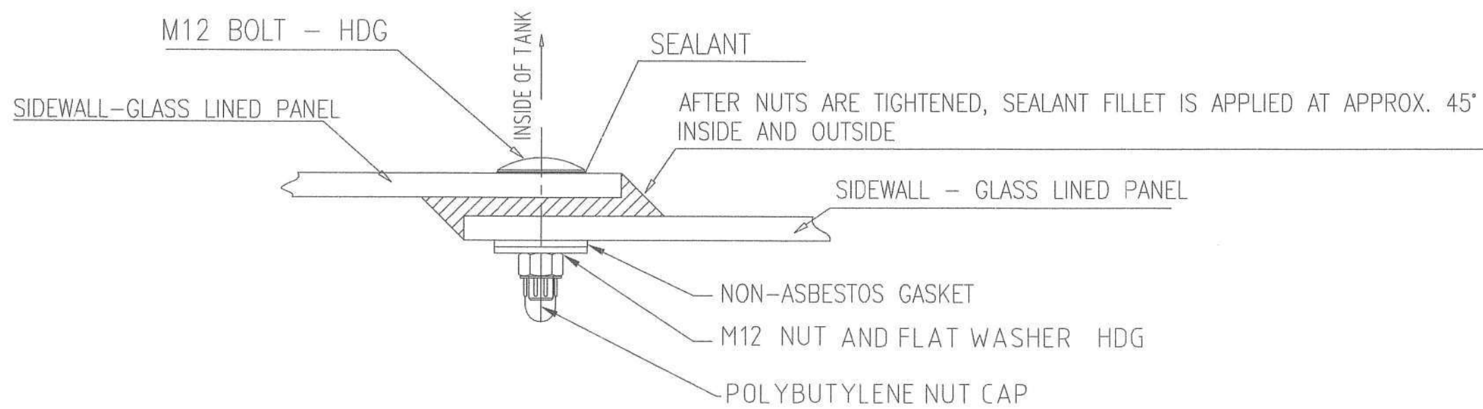
SIDEWALL SEALANT DETAILED
