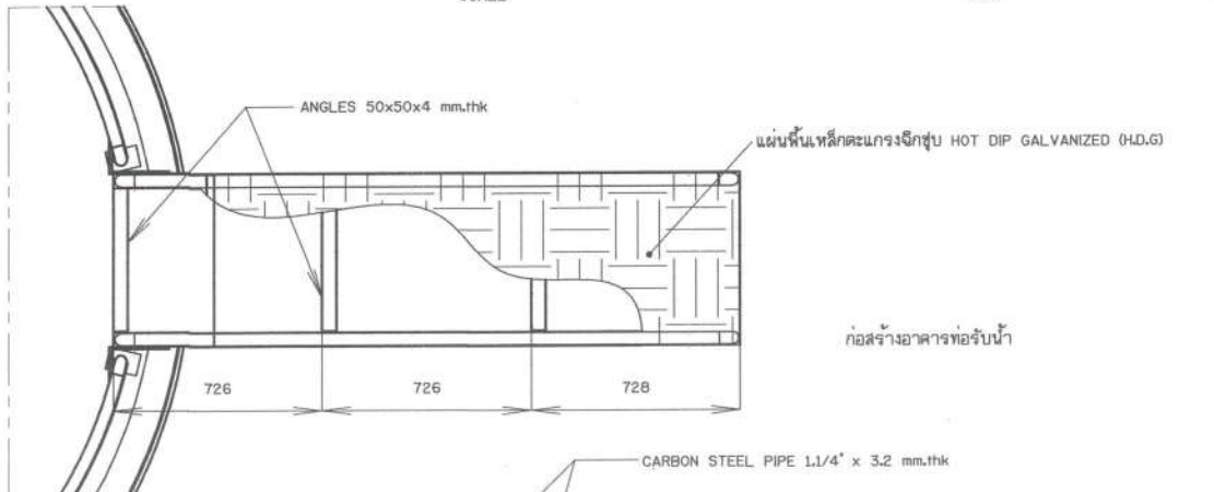
DETAIL TANK + LADDER SCALE 1:30
