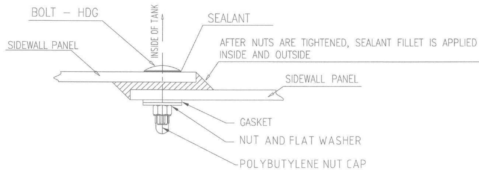
SIDEWALL SEALANT DETAILED
