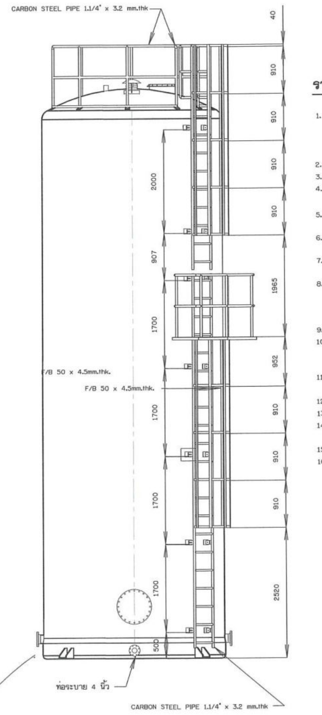
DETAIL TANK + LADDER SCALE 1:75
