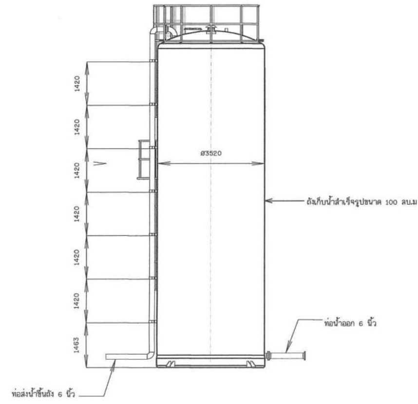
WATER STORAGE TANK MODEL SCALE 1:125
