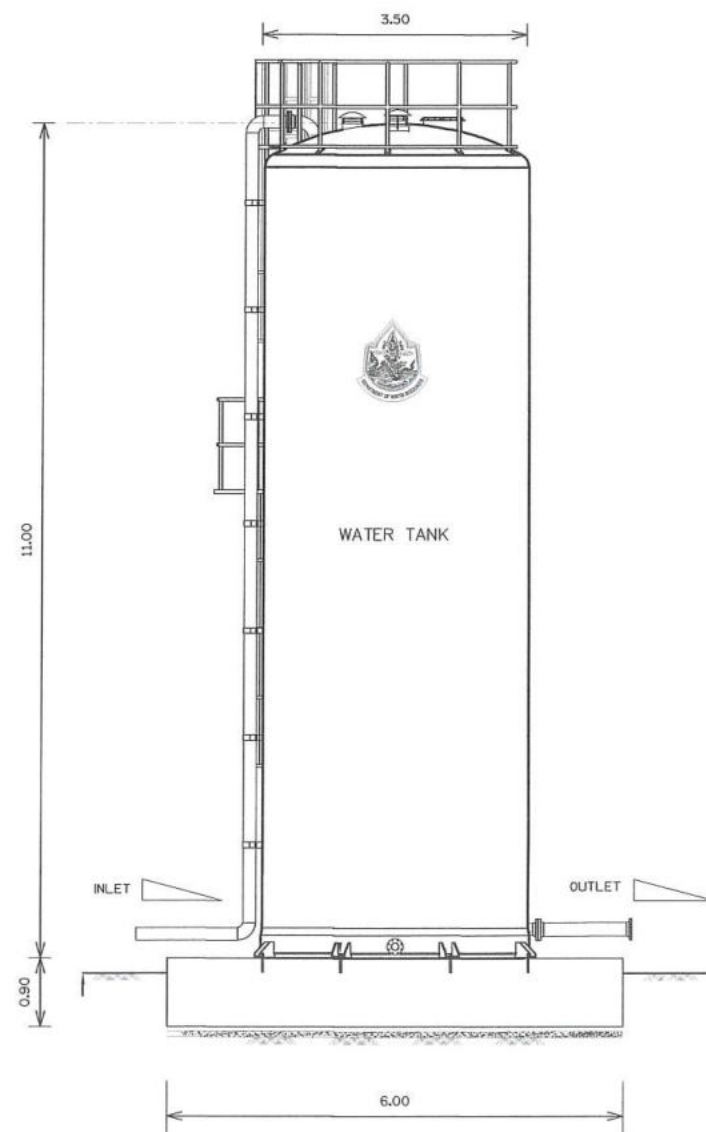
FOOTING PLAN (WTF-100000V-D3.50) SCALE 1 : 75
