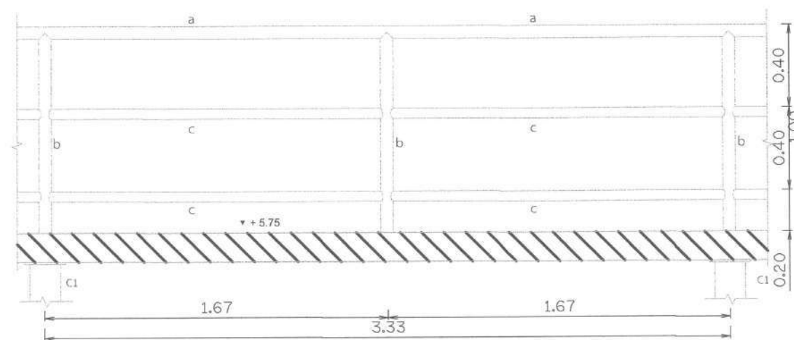
DETAIL : GUARD RIAL (OUTSIDE) SCALE (A3) 1 : 25
