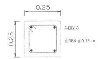
C1, C2, C3 SCALE (A3) 1:15
