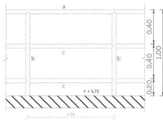
DETAIL : GUARD RIAL (SPIRAL STAIRCASE) SCALE (A3) 1 : 25
