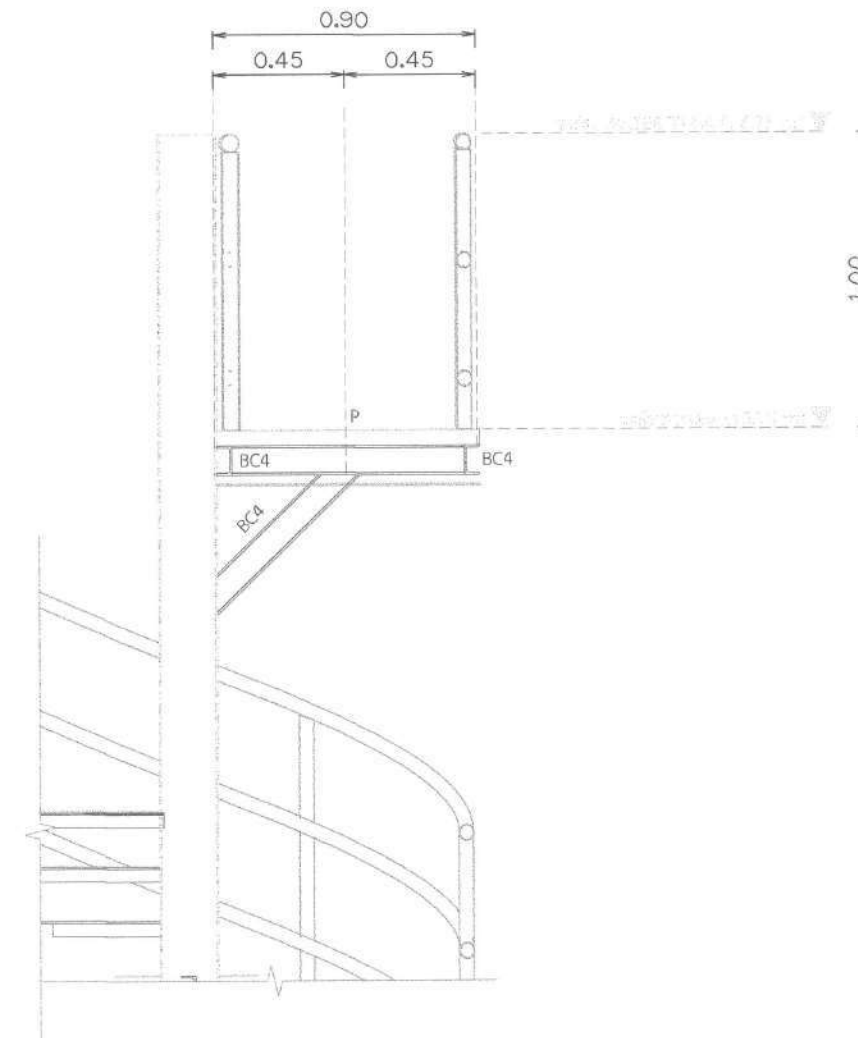
DETAIL A : SECTION X-X SCALE (A3) 1 : 25
