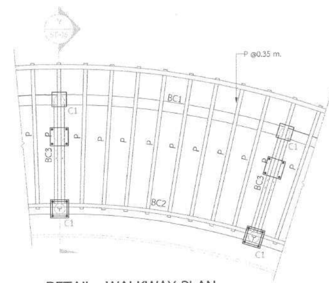
DETAIL : WALKWAY PLAN SCALE (A3) 1:30
