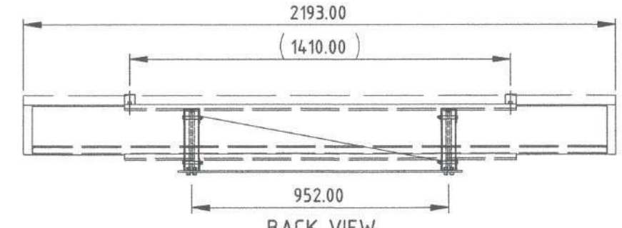
BACK VIEW SCALE 1:20
