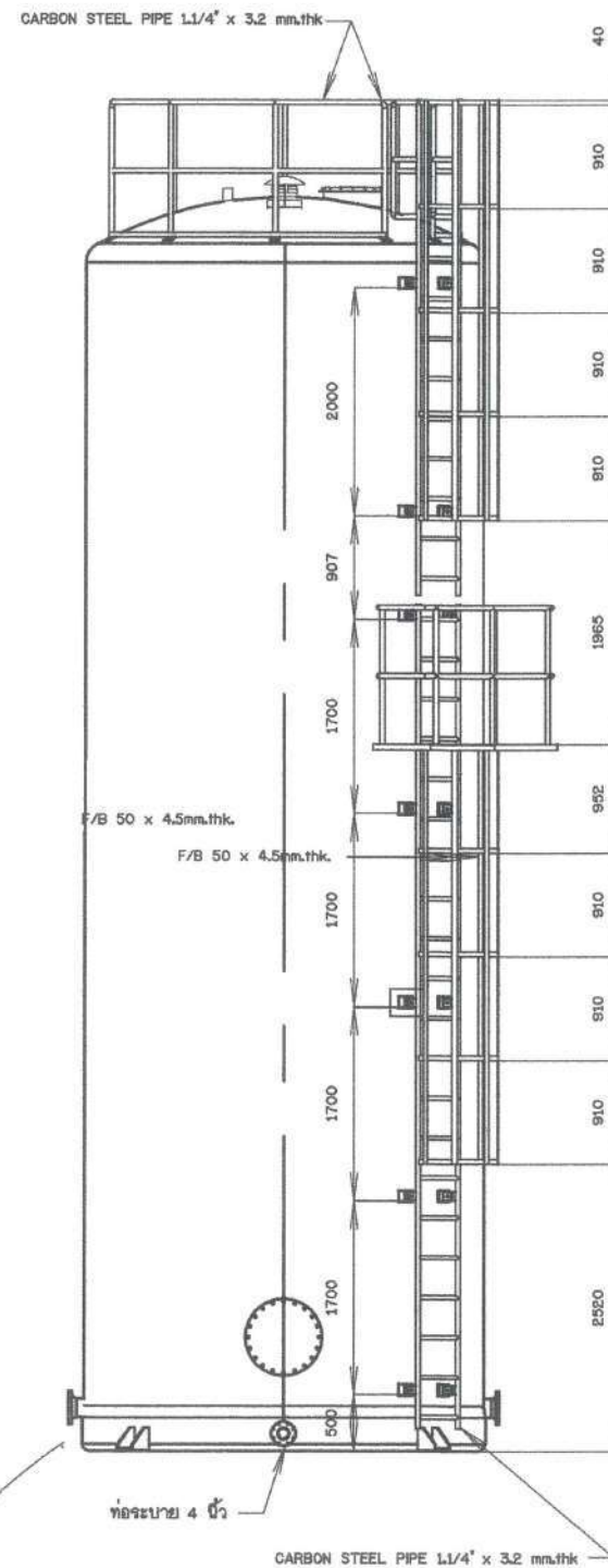
DETAIL TANK + LADDER SCALE 1:75
