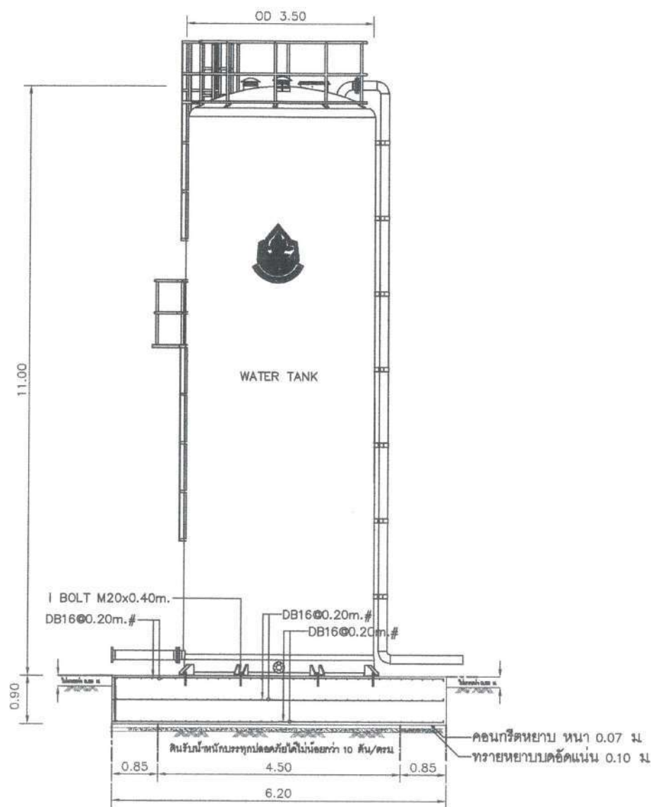
SECTION (A) SCALE 1 : 100
