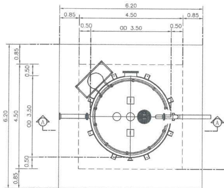
FOOTING PLAN (WTF-100000V-D3.50) SCALE 1 : 75
