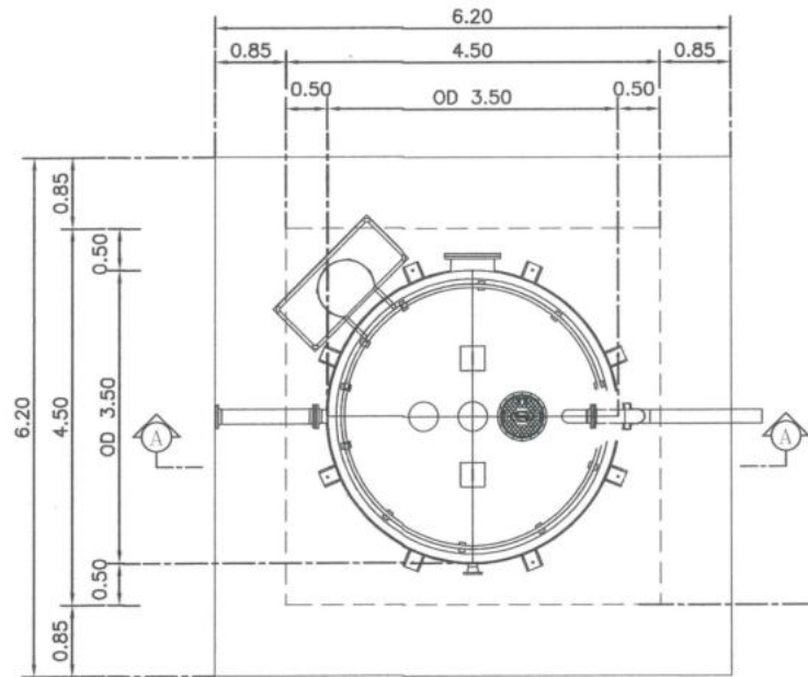
FOOTING PLAN (WTF-100000V-D3.50) SCALE 1 : 75
