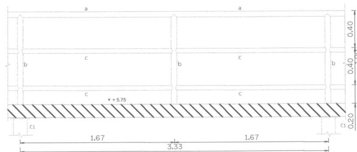
DETAIL : GUARD RIAL (OUTSIDE)
