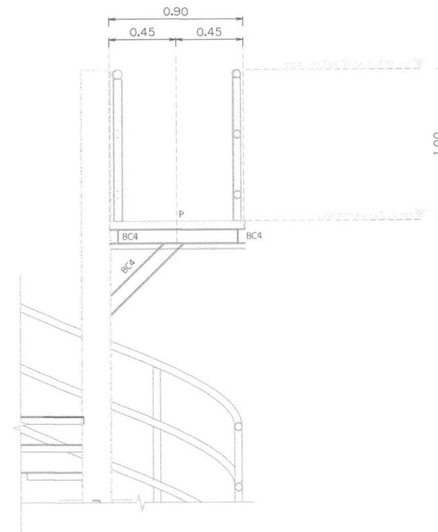
DETAIL A : SECTION X-X
