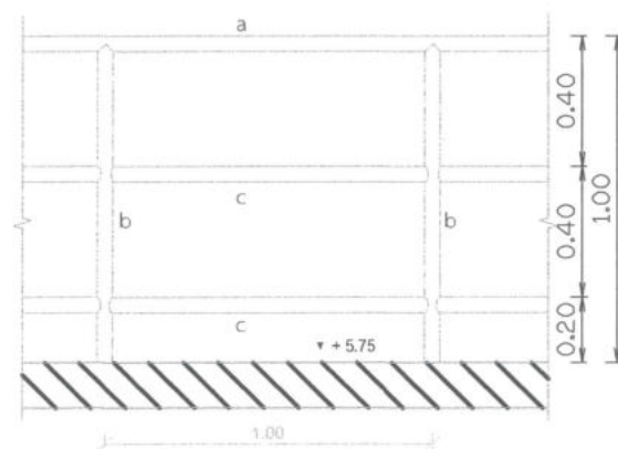
DETAIL : GUARD RIAL (SPIRAL STAIRCASE)
