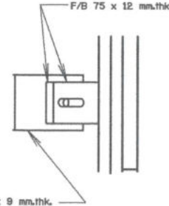
DETAIL A SCALE 1:10
