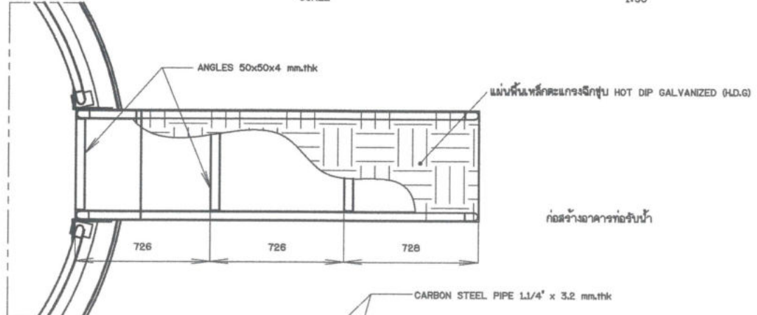
DETAIL TANK + LADDER SCALE 1:30
