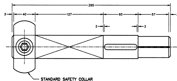
STANDARD SAFETY COLLAR
