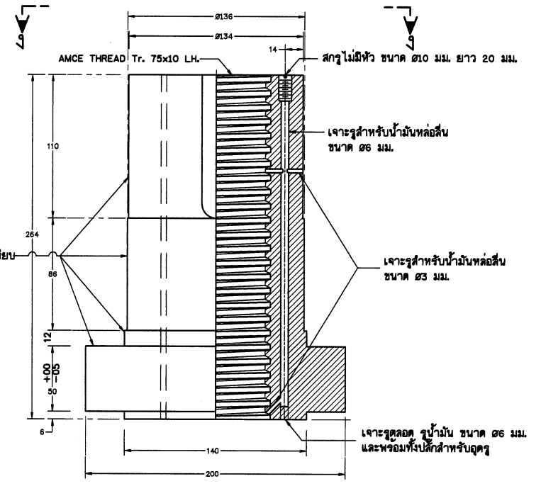
LIFTING NUT
