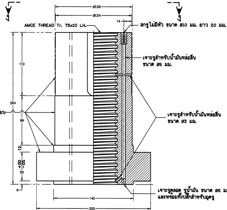
LIFTING NUT
