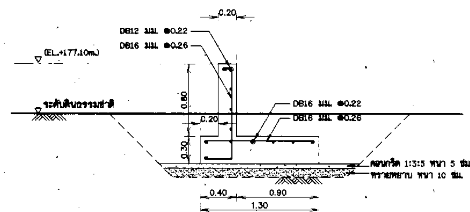
DETAIL FW
