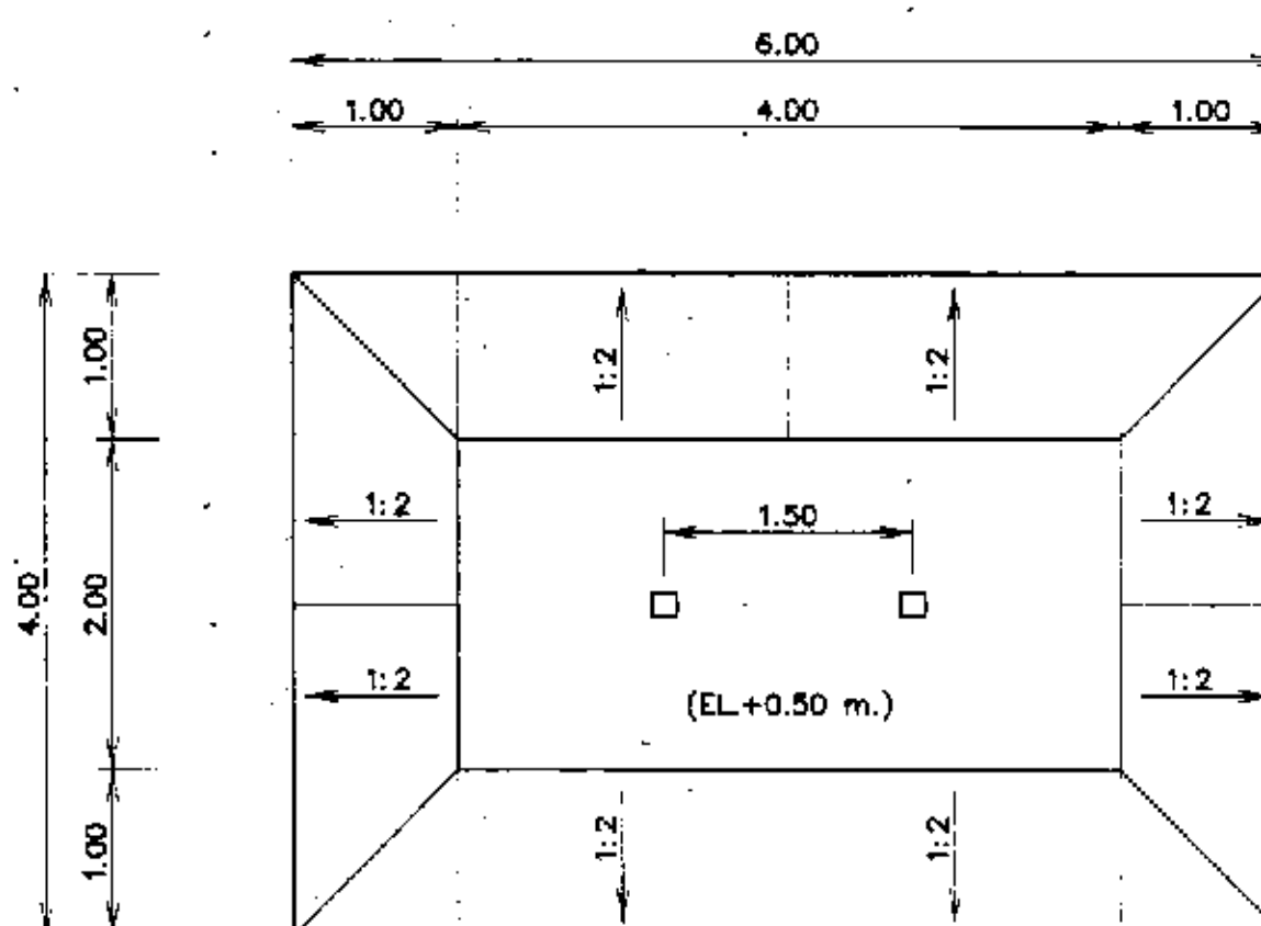
DETAIL FW
