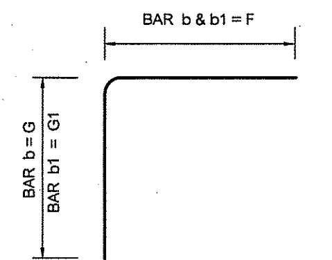
BENDING DETAILS FOR BARS b & b1 NOT TO SCALE
