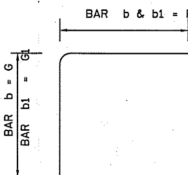
BENDING DETAILS FOR BARS b & b1 NOT TO SCALE
