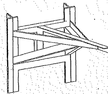
ISOMETRIC
