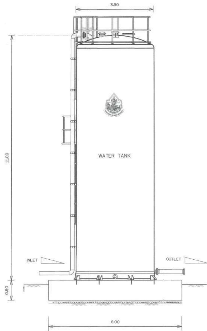
SECTION (A) SCALE 1 : 100
