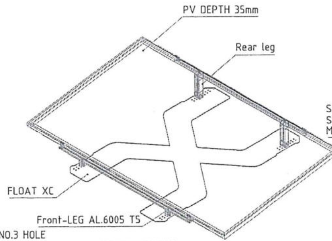
ISOMETRIC VIEW SCALE 1:20
