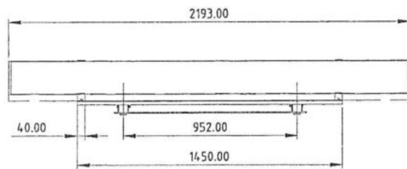
FRONT VIEW SCALE 1:20
