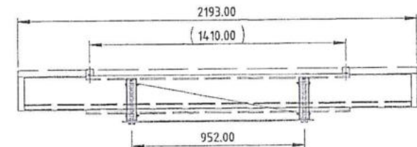
BACK VIEW SCALE 1:20
