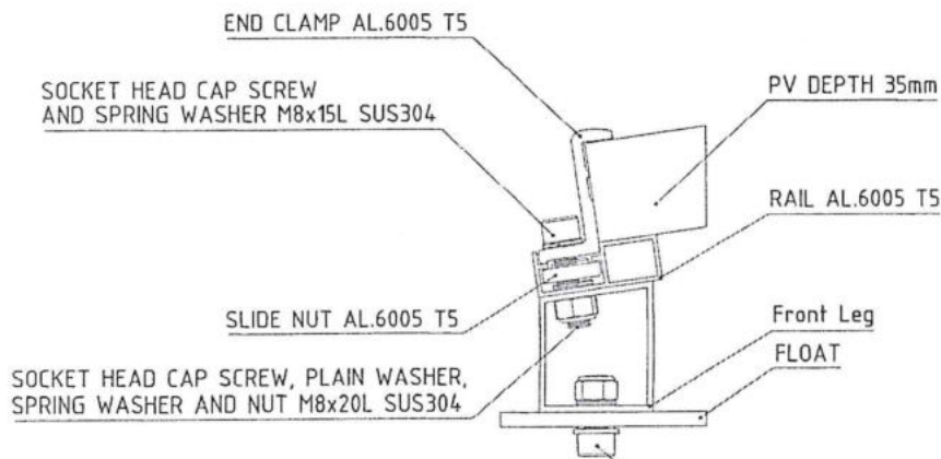
DETAIL - A SCALE 1:2
