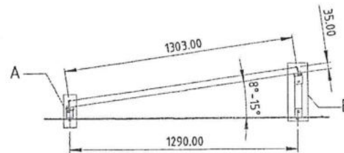
SIDE VIEW SCALE 1:20
