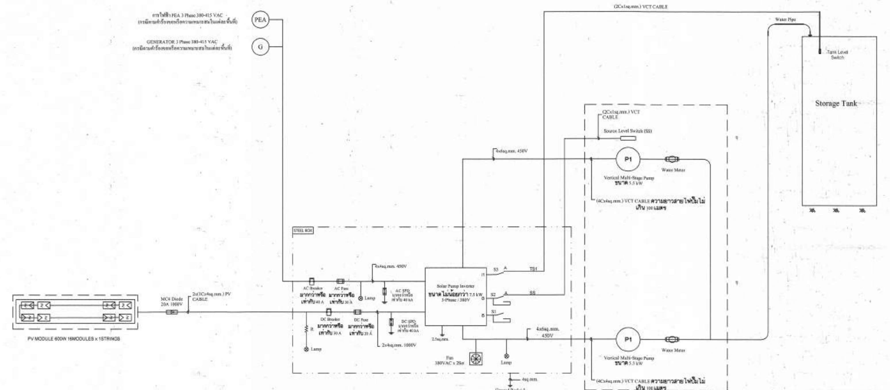
SINGLE LINE DIAGRAM (5.5kW-Pump x 2Units)
