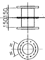
TYPICAL DOUBLE FLANGED CONNECTOR ARRANGEMENT
