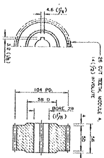
② PINION CAST IRON NOT TO SCALE
