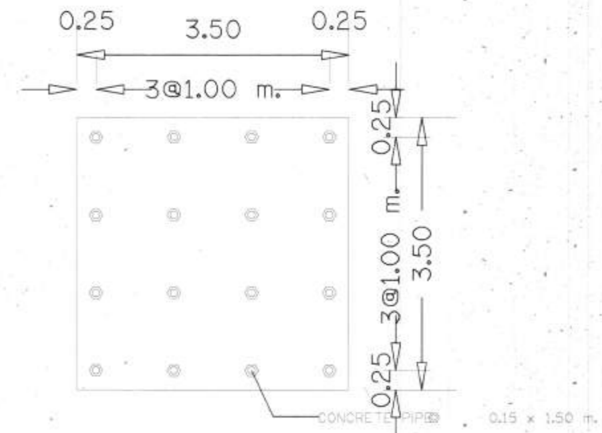
PLAN OF FOUNDATION SCALE : 1:100
