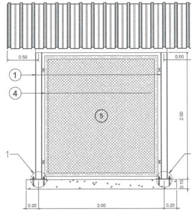
ELEVATION C
