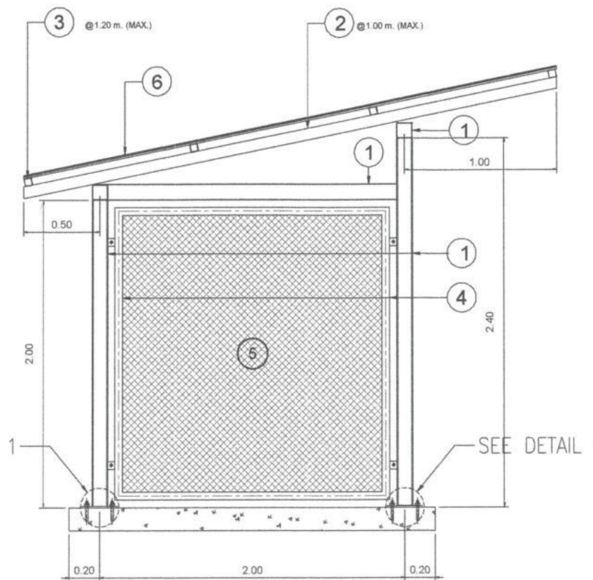
ELEVATION D
