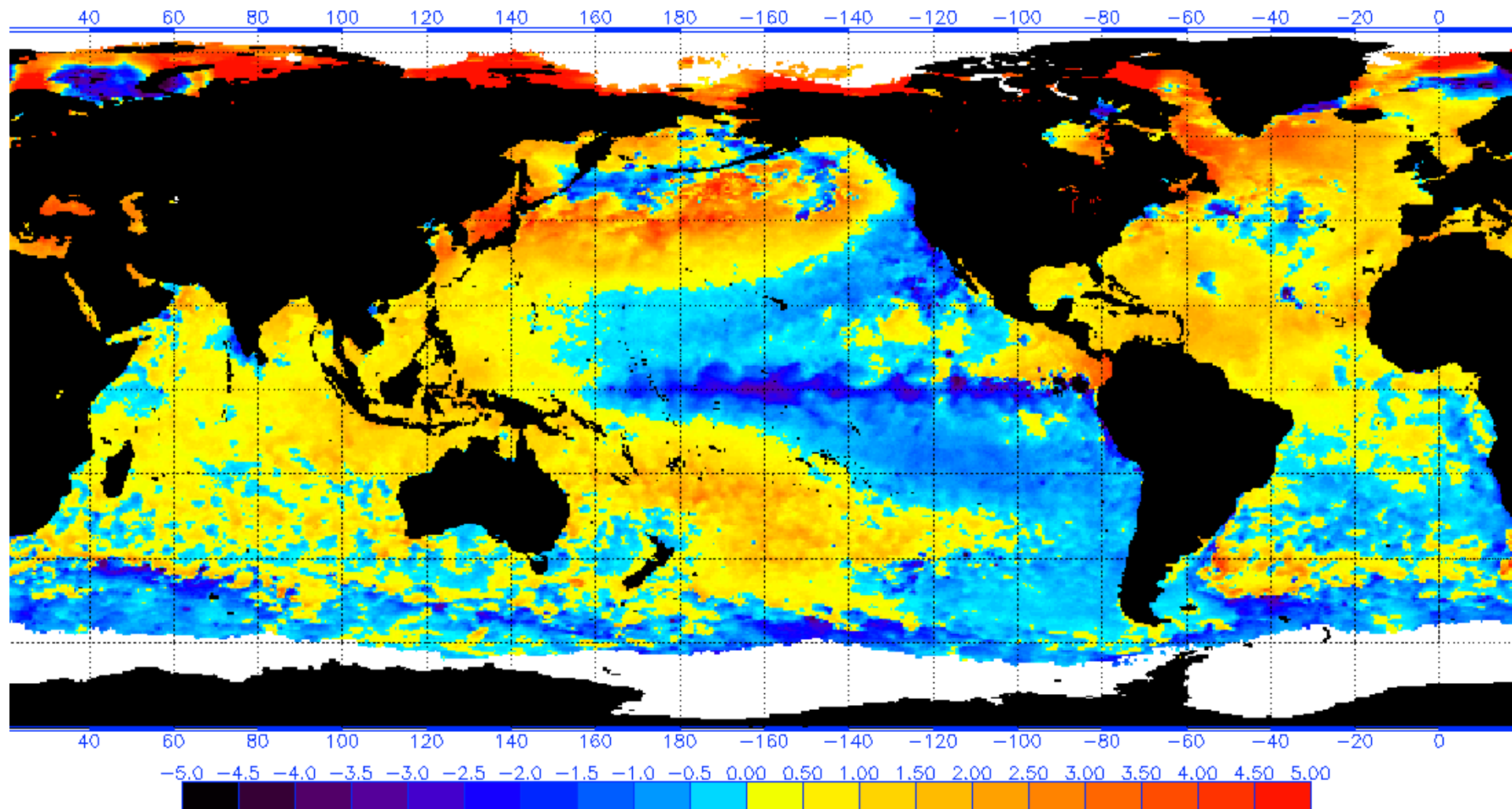
NOAA/NESDIS 50 KM GLOBAL ANALYSIS: SST Anomaly (degrees C), 8/30/2010 (white regions indicate sea-ice)
